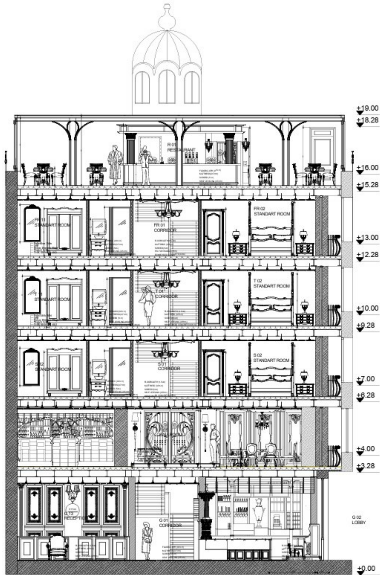
A-A SECTION 1:50 SCALE
