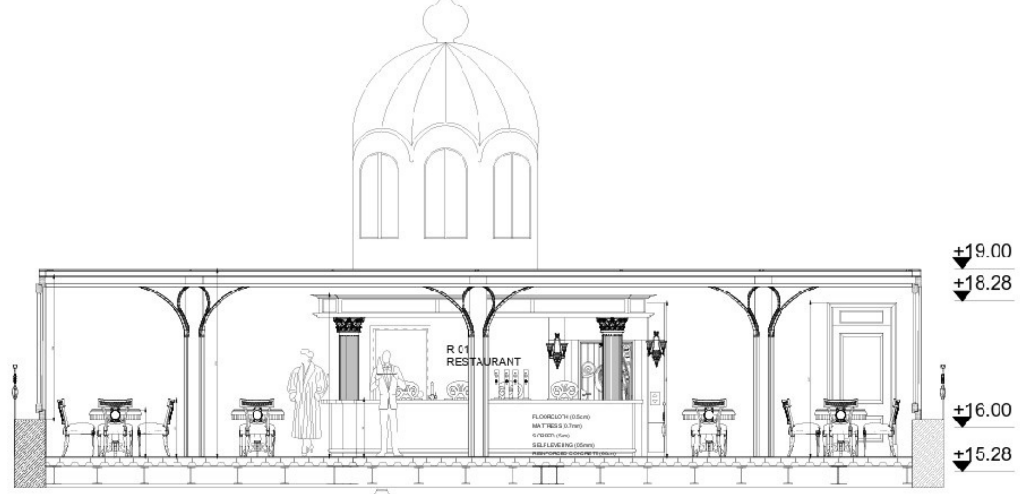
Restaurant B-B Section Scale: 1/20
