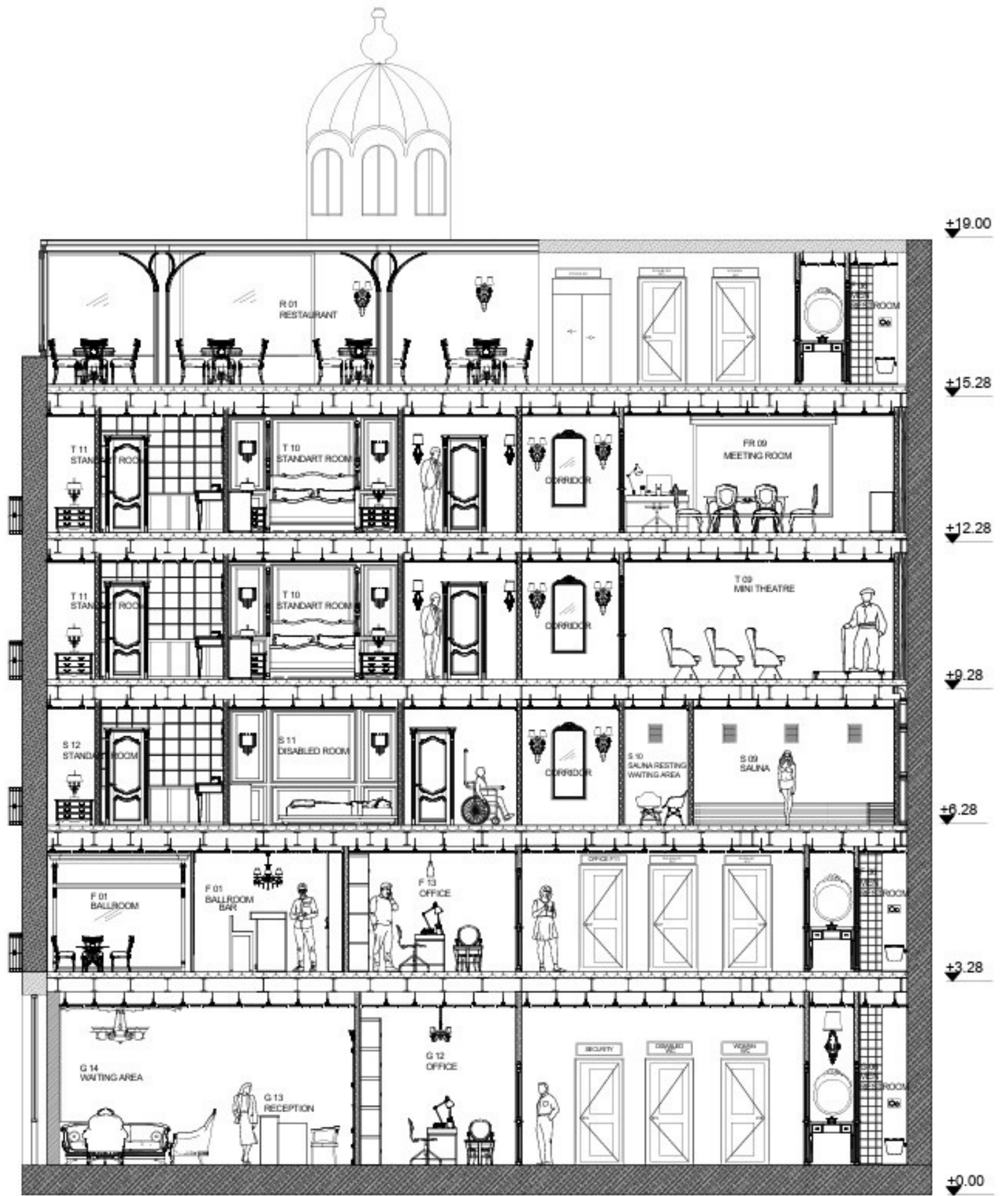
BB SECTION 1:50 SCALE
